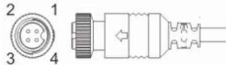
Aviation RS765-4(Female)
